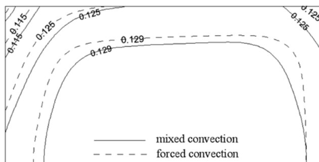
Fig. 13. Moisture profiles obtained by mixed and forced convection models in Re=200 ( t=8\frac{1}{4} hr).
