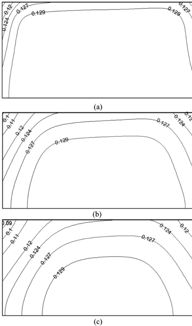
Fig. 5. Moisture content distributions (kg moisture/kg dry) during drying. (a) t=2\frac{1}{2} hr, (b) t=9 hr, (c) t=15\frac{1}{2} hr
