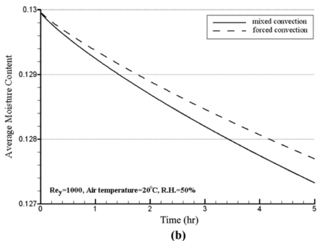
Fig. 15. Drying curve for mixed and forced convection models. (a) Re=50 (b) Re=1,000
